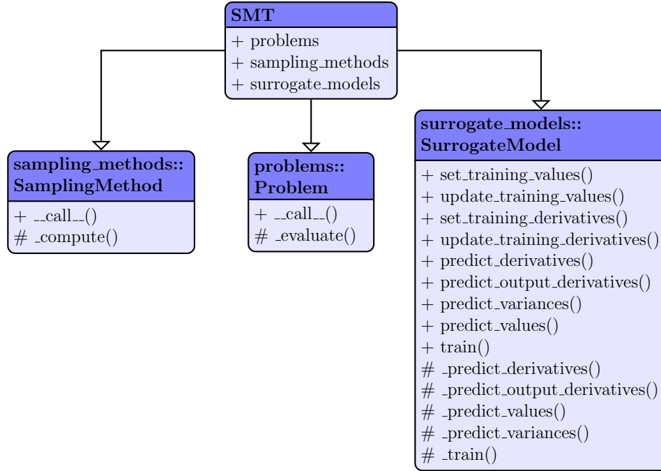
Figure 1: Architecture of SMT.
