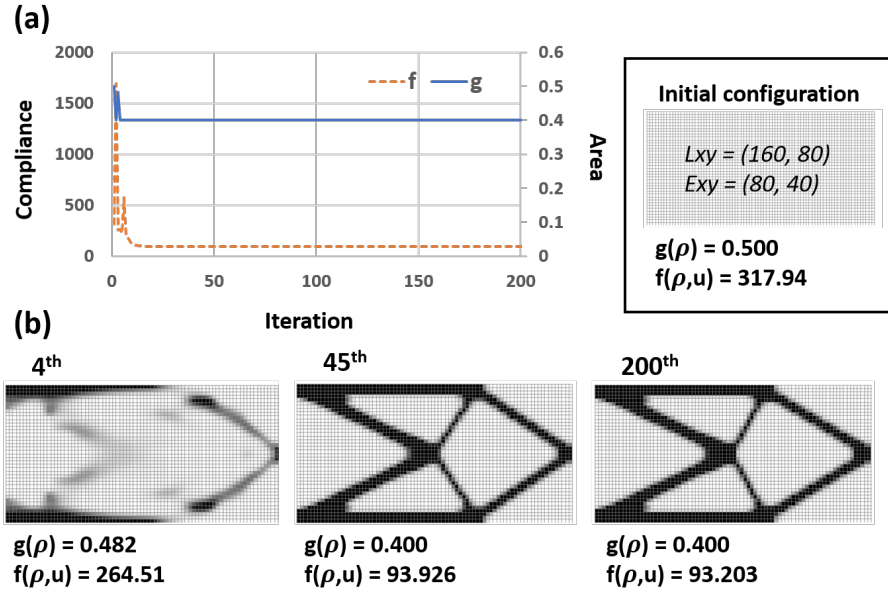
Fig. 6 Numerical results of SIMP. (a) a convergence profile with initial configuration where the number of meshes to each direction are specified (b) a material configuration, area fraction (g) and compliance (f) found during at the 4 th , 45 th , and 200 th iterations.
