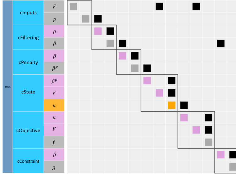
Fig. 4 Design structure matrix of SIMP method.
