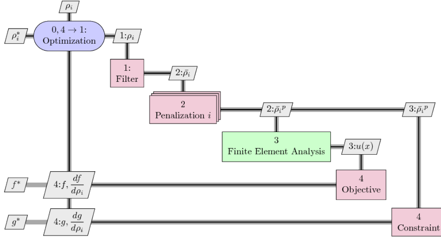
Fig. 1 XDSM diagram of the SIMP method
