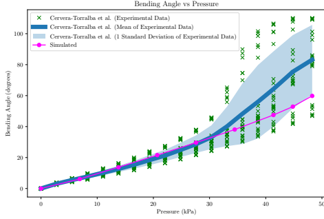
Fig. 3: The actuator bending angle (degrees) is plotted against the chamber pressure (kPa) for the simulated data (magenta circles) and the pre-existing experimental data (green) [6].
