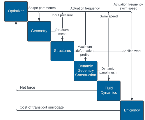
Fig. 2: Model Flowchart
