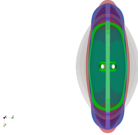
Fig. 5: The cross sections of the baseline (gray), high-level parameterization (red), multilevel parameterization (blue), and multilevel with updated model parameters (green) optimization results.
