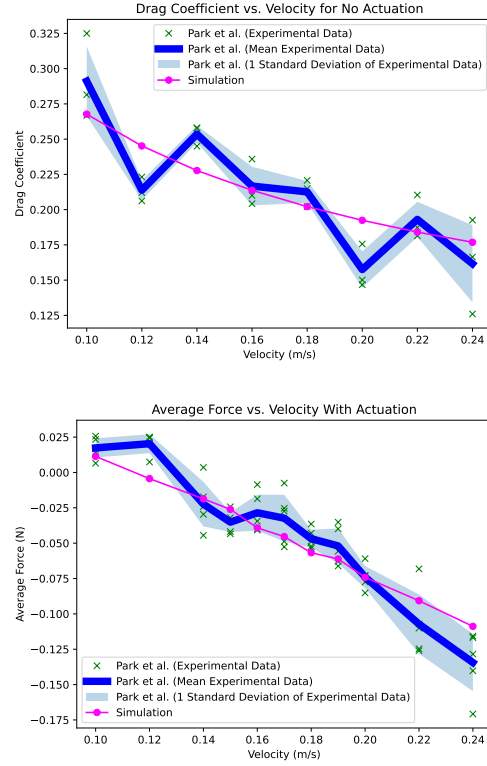
Fig. 4: Comparisons between simulation (magenta) and pre-existing experimental data [25] (green) to estimate the fluid dynamics model parameters
