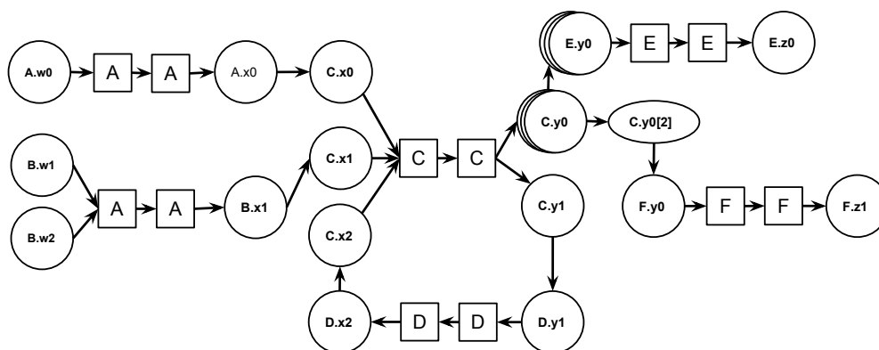
Figure 1: Dependency graph for a notional problem, using Pate et. al's proposed structure
