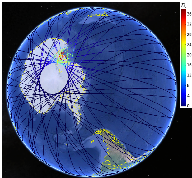
Figure 9: Ground trace of the satellite trajectories for all the design points colored by communications bit rate.
