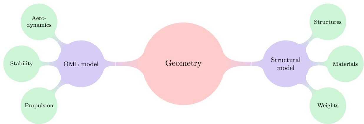
Figure 1: Illustration of how each discipline interacts with the geometry. The aerodynamic mesh is linked to the OML model through the mesh movement algorithm. Stability coefficients and their derivatives are computed by the flow solver, and the quantities computed by the propulsion model determine the inlet and outlet CFD boundary conditions. The materials discipline provides stiffness matrices for the shell elements used in the structural analysis, and a significant portion of the weight build-up depends on the airframe.
