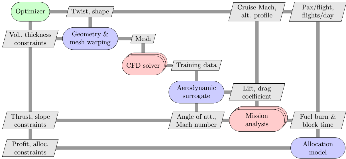
Figure 2: Extended design structure matrix (XDSM) diagram of the data flow in the allocation-mission-design optimization.
