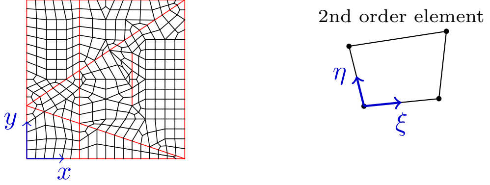
Figure 4: Global (left) and local (right) coordinate frames for the elliptical smoothing.
