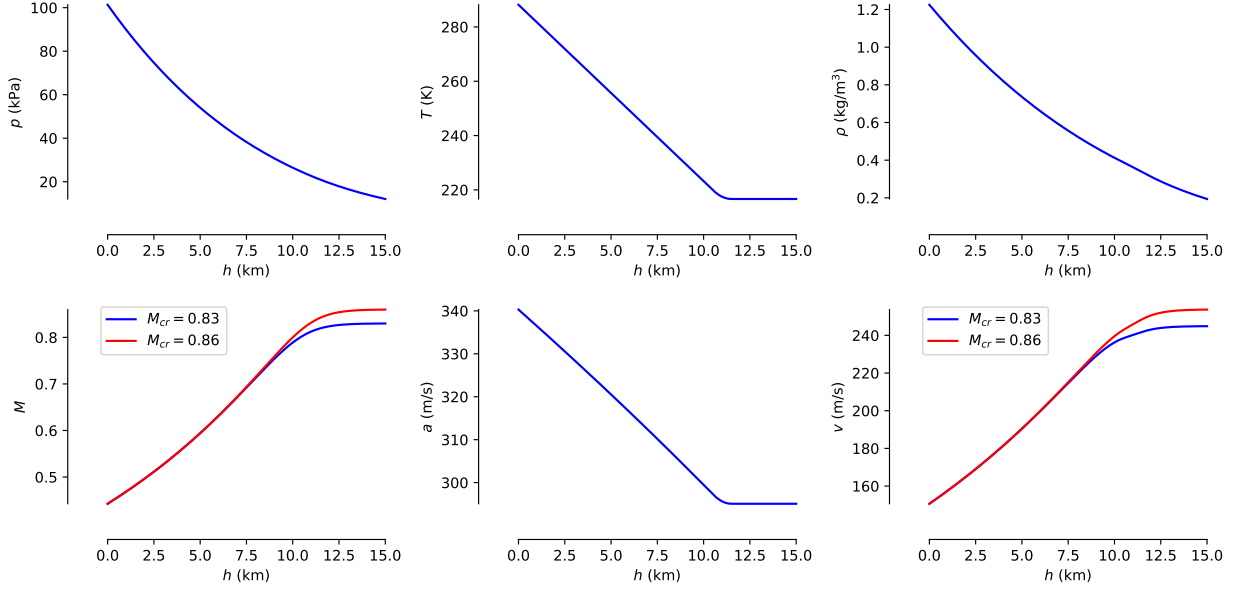
Fig. 3 Pressure, temperature, density, and speed of sound are computed using atmospheric models. For the Mach number, we assume a constant indicated airspeed climb at 300 knots until the cruise Mach number is reached.
