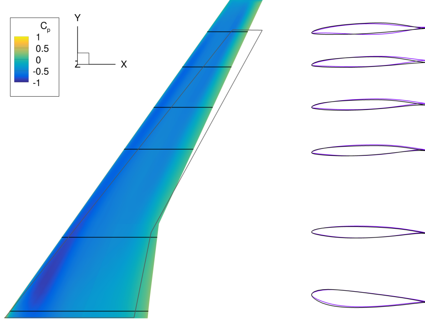
Fig. 7 Initial (purple) and optimized (black) wing design. The grey outline depicts the planform for the initial wing.
