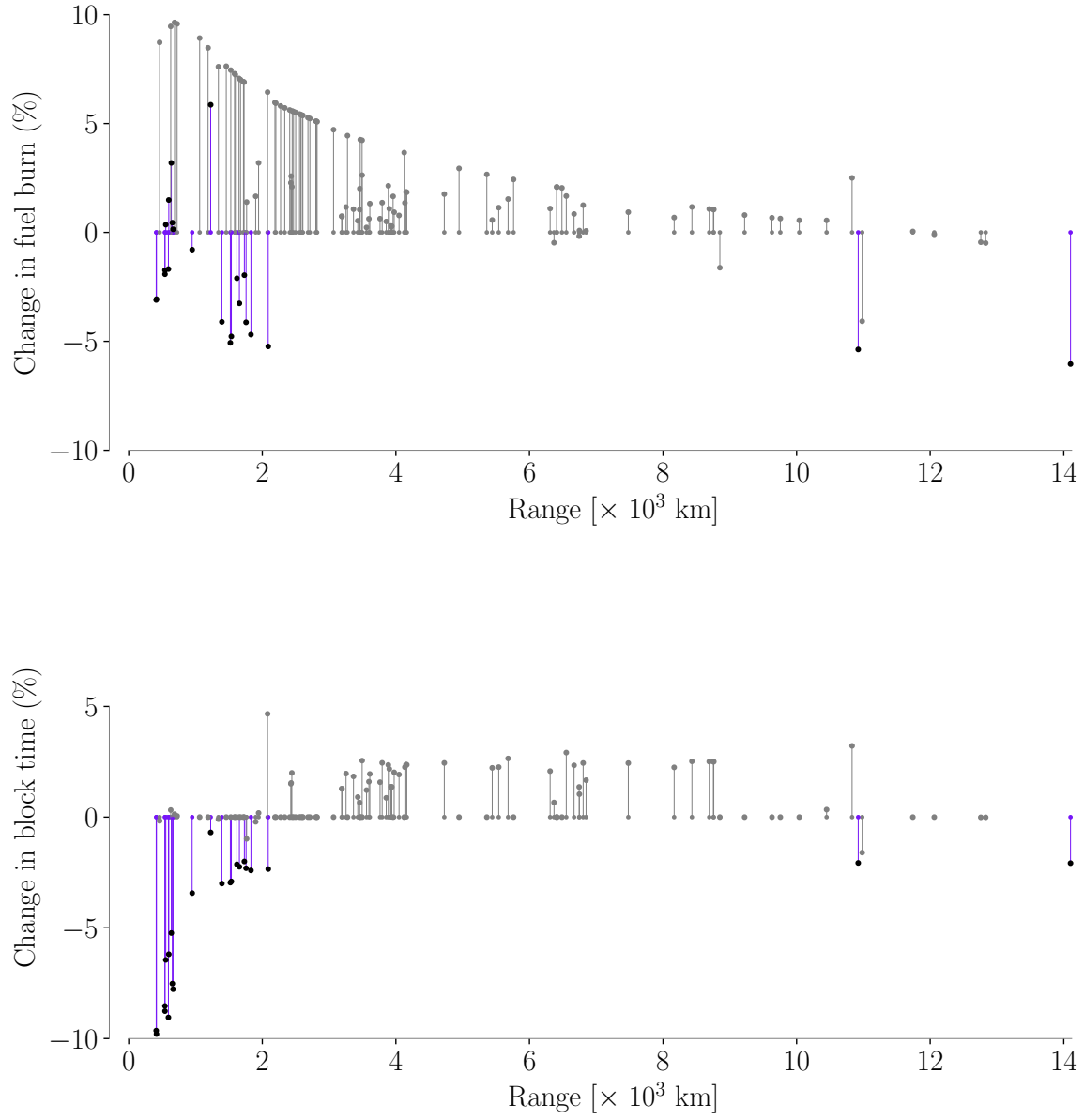
Fig. 10 Missions on which the CRM is not flown are in grey, values for the initial design are in purple, and values for the optimized design are in black.
