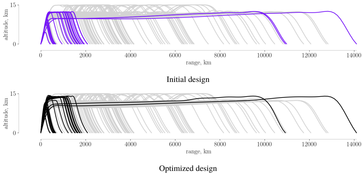
Fig. 9 The altitude profiles for: routes on which the CRM is not flown (grey), the initial design (purple), and the optimized design (black).
