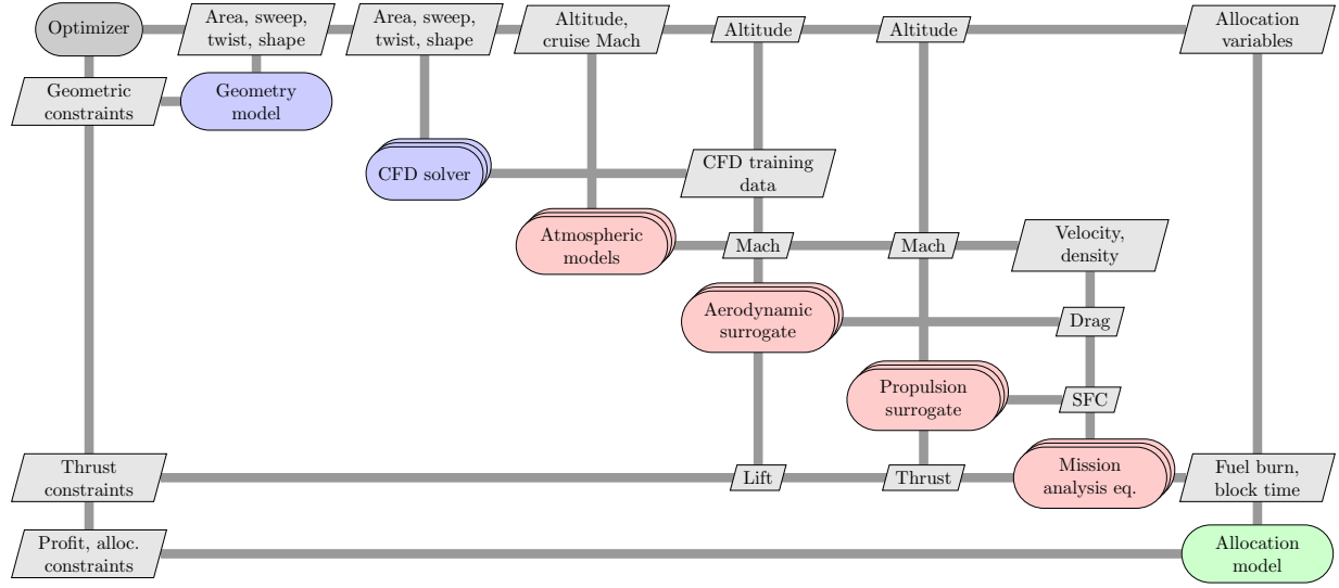
Fig. 1 Design structure matrix showing the design (blue), mission (red), and allocation (green) parts of the model and the dependencies between them.
