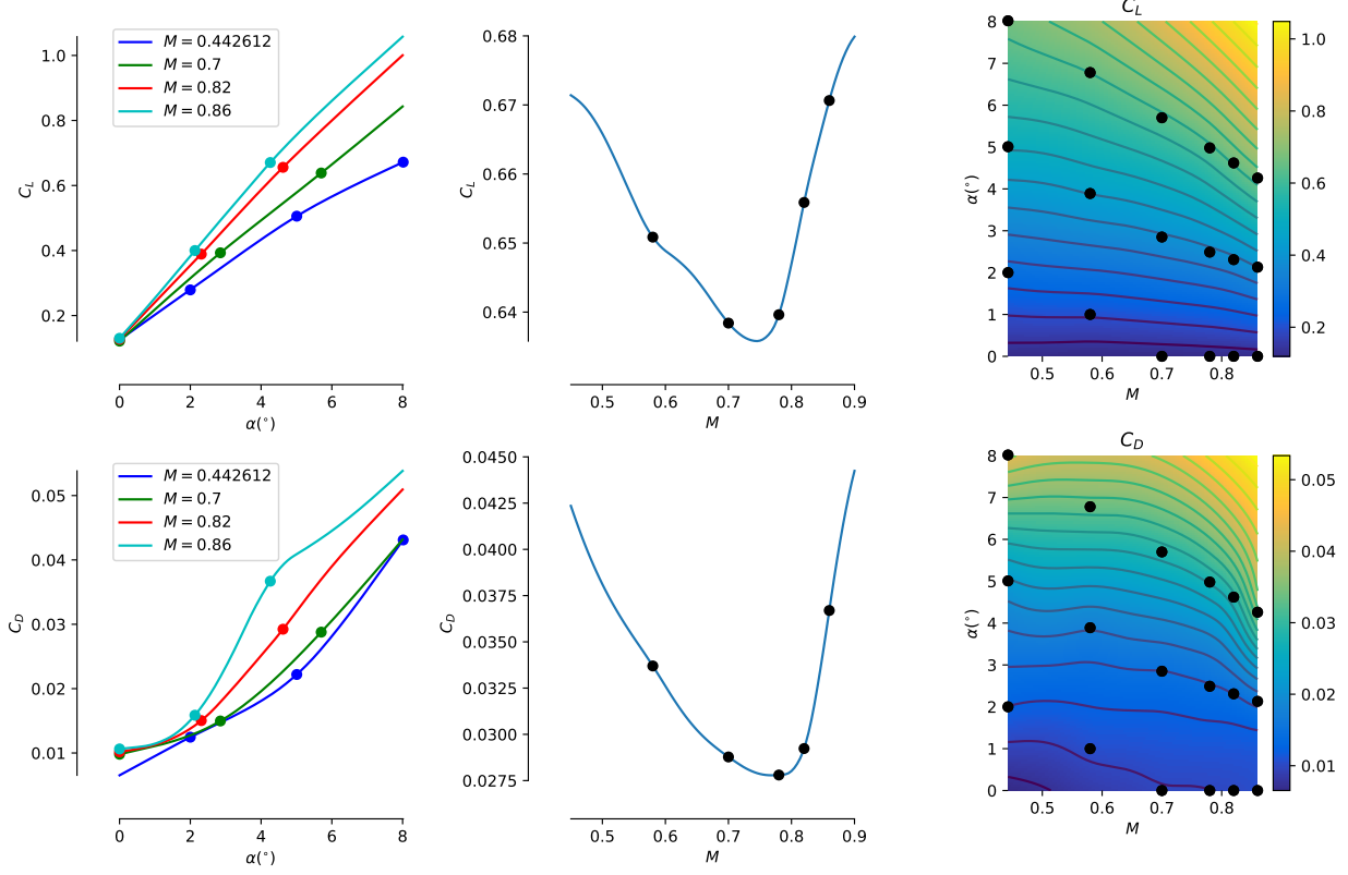
Fig. 4 1-D slices and contour plots for the aerodynamic surrogate model for the CFD solver. The plots in the middle represent a diagonal slice passing through the top row of training points in the contour plot.
