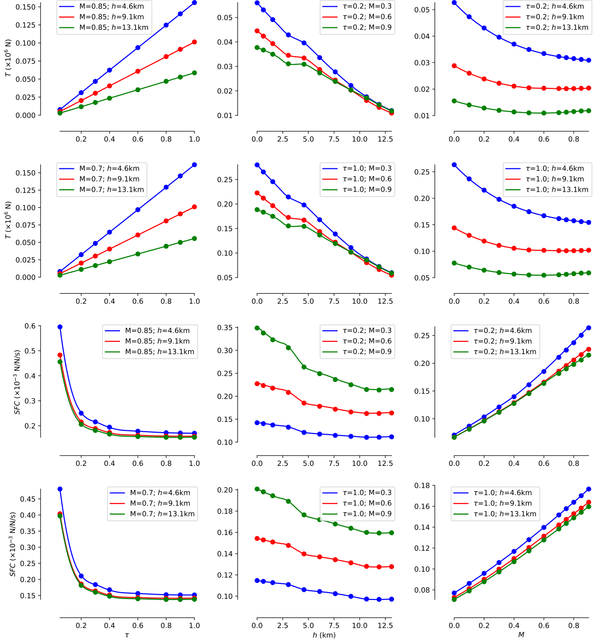
Fig. 5 1-D slices versus of thrust and specific fuel consumption versus throttle setting, altitude, and Mach number.
