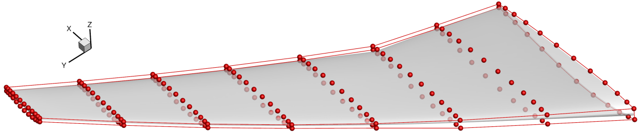
Fig. 2 The Common Research Model (CRM) wing [51] enclosed in a free-form deformation block with the control points shown in red.
