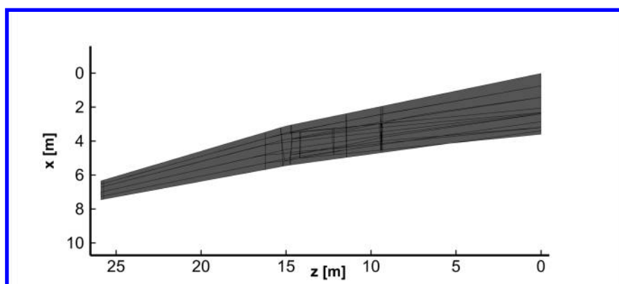
Figure 3. Top view of the truss-braced wing configuration.
