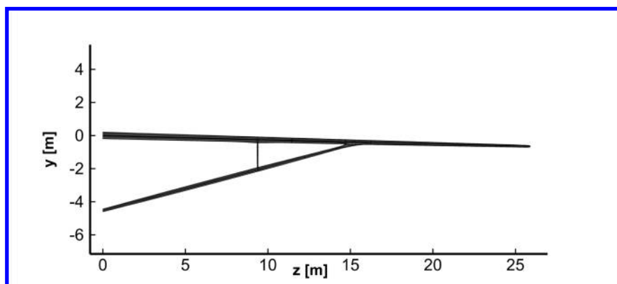
Figure 4. Front view of the truss-braced wing configuration.
