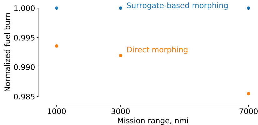
Figure 9. The direct morphing approach yields the biggest gains in the long range mission, where we see a 1.5% decrease in fuel burn. This effect is mostly due to the direct morphing optimization being able to tailor the structural thickness distribution and the morphing twist simultaneously to find the optimal balance between load alleviation, weight, and aerodynamic performance.
