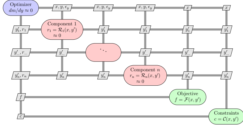
Fig. 5 SURF architecture[42] . Model solves the residual equations to tolerances \epsilon_y provided by the optimizer.
