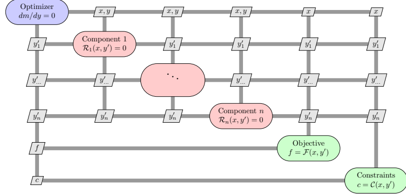
Fig. 4 Modified full-space architecture [42].
