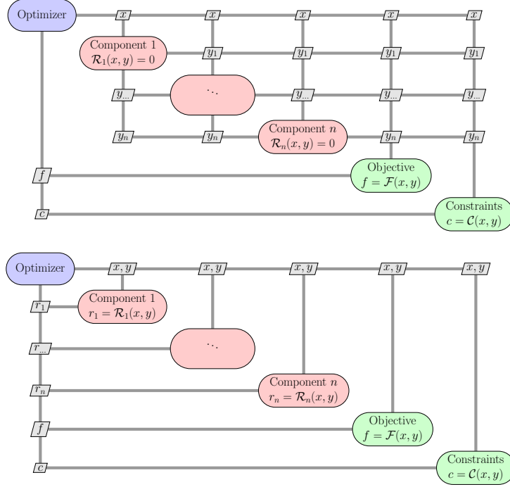
Fig. 2 Reduced-space versus full-space formulation for a model containing implicit state variables [1].
