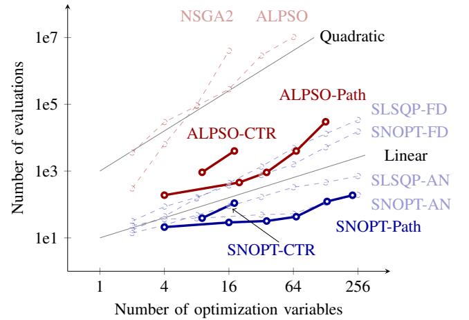
Fig. 2. Optimization algorithm scaling with the number of optimization variables, computed using the multi-dimensional Rosenbrock problem (shown in dashed lines), as well as using the proposed path and CTR optimization problems (shown in solid lines). For all cases, the gradient-free optimizers (ALPSO, NSGA2) scale quadratically or worse, while the gradient-based optimizers (SNOPT, SLSQP) scale linearly with finite-difference derivatives (FD), and better than linearly with analytic derivatives (AN) [31].
