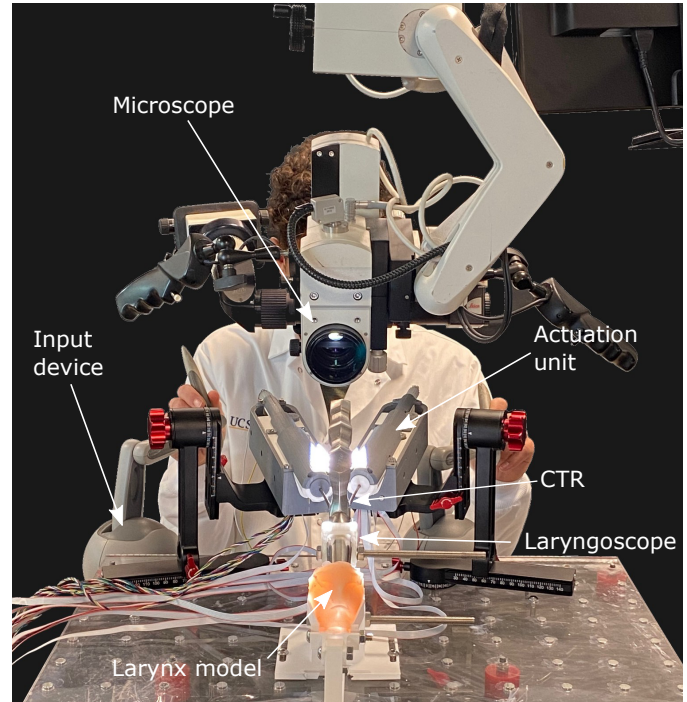
Fig. 1. Proposed dual-CTR system for micro-laryngeal surgery. This system uses a microscope to visualize the larynx through a laryngoscope and the CTRs are teleoperated using two 6-DOF input devices.
