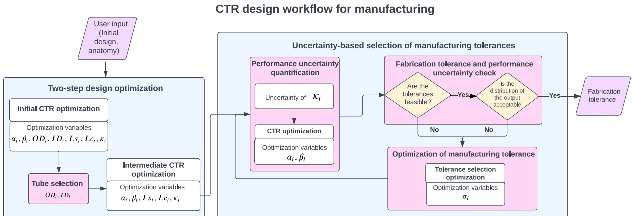
Fig. 3. Illustration of the proposed CTR design workflow for manufacturing. The workflow consists of two main parts. The first block is the two-step design optimization where two design optimization processes are performed in order to finalize the tube design for shape setting. The next block aims to determine the fabrication tolerance for tube curvature, \kappa_i , through an uncertainty-based selection of manufacturing tolerances.
