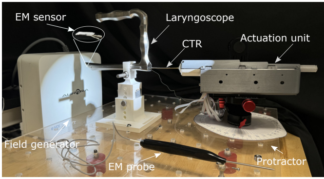
Fig. 10. The experimental setup for orientability evaluation includes a single CTR system with a field generator and an EM sensor attached to the tip of the CTR. The protractor and EM probe are used for calibrating the robot's base frame.
