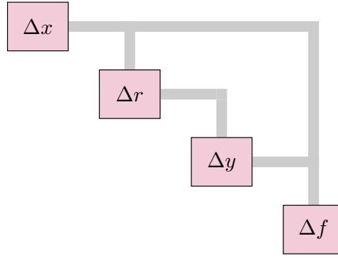
Figure 7: Dependence of the variations in the design variables, residuals, states and quantities of interest for the linearized system
