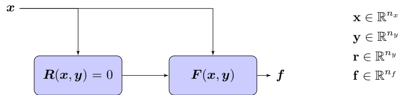
Figure 4: Definition of the variables involved at the solver level, showing the dependency of the quantity of interest on the design variables, both directly and through the residual equations that determine the system states
