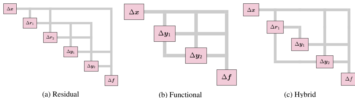
Figure 10: The different approaches for handling coupled multidisciplinary systems
