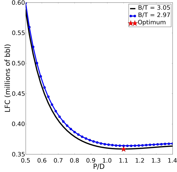
Figure 8: Variation of the LFC as a function of P/D at D/T = 1.2 and for three different B/T values.
