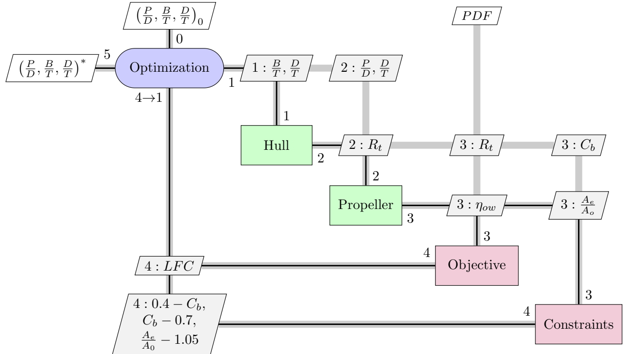
Figure 5: Data and process flow diagram for the hull-propeller design optimization process.
