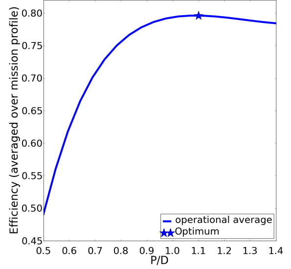
Figure 9: Variation of the overall efficiency averaged over the entire operational profile as a function of P/D . D/T and B/T are both at the optimum values of 1.2 and 3.05, respectively.
